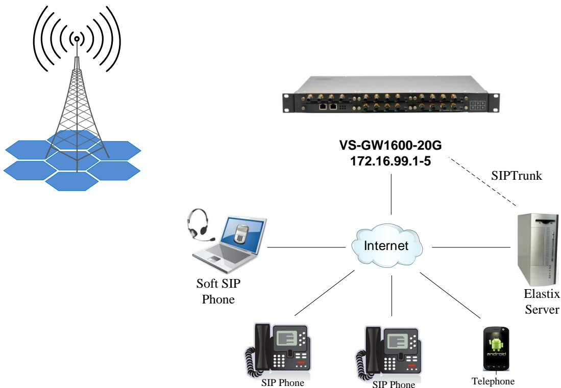
Figure 1-2-1 Topological Graph
