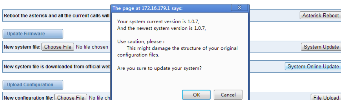
Figure 2-5-2 Prompt Information
