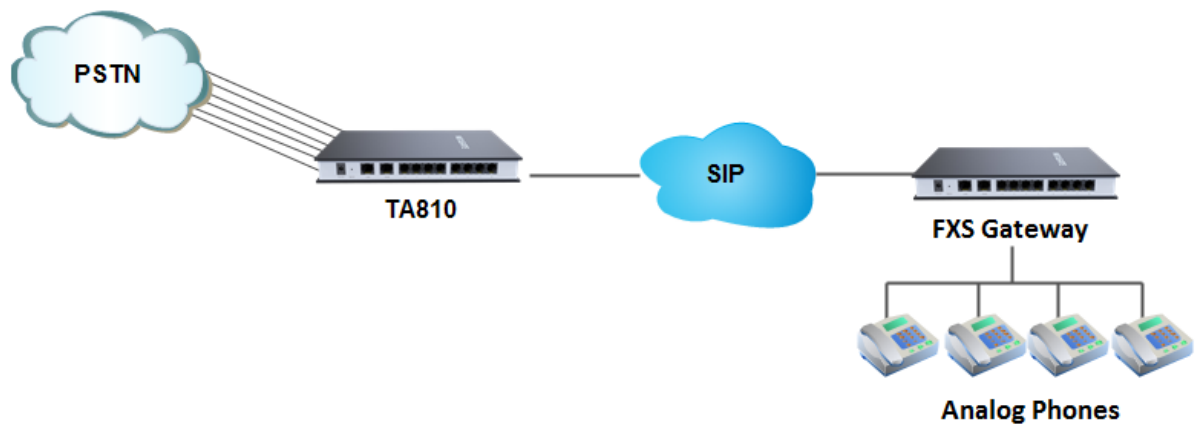
Figure II-2 Connect TA810 and FXS Gateway
