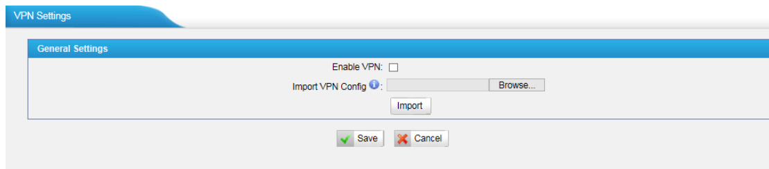
Figure 8-6 VPN Settings
