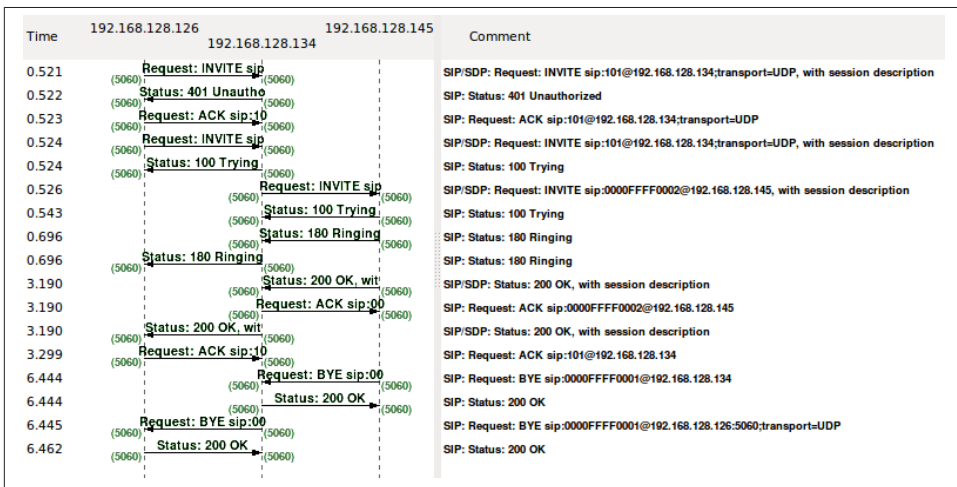
Figure 5-2. SIP dialogs
